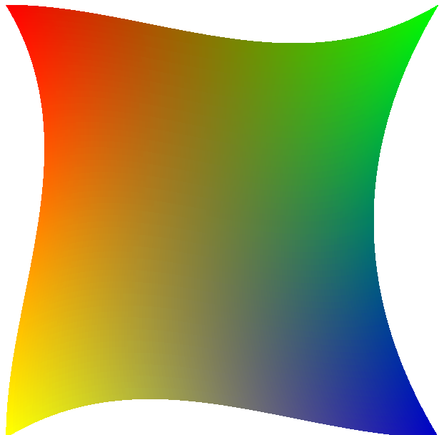
CoonsPatchMesh()
